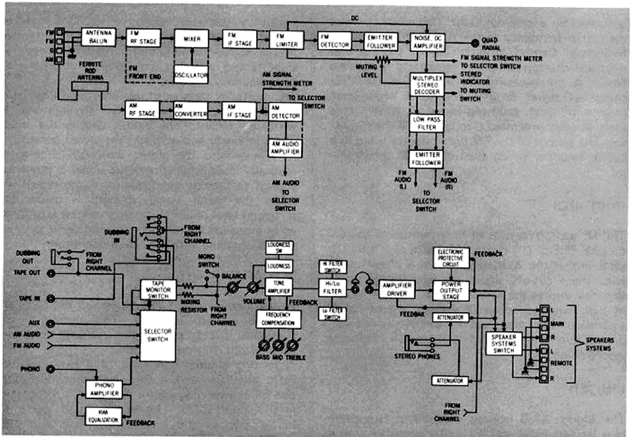
Figure 8. Functional Block Diagram
