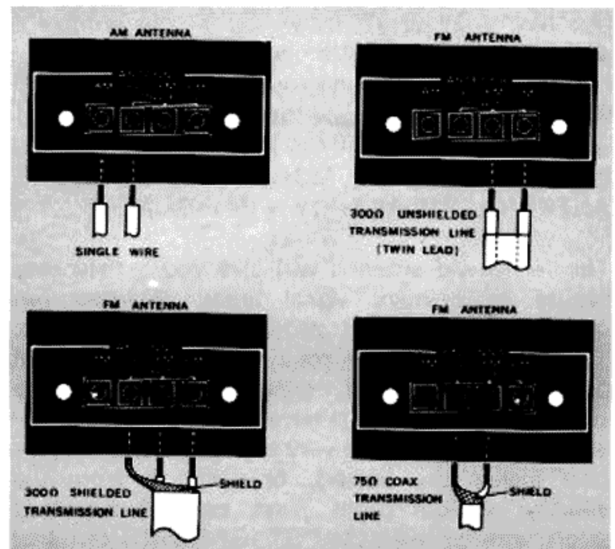
Figure 3. FM/AM Antenna Connection
