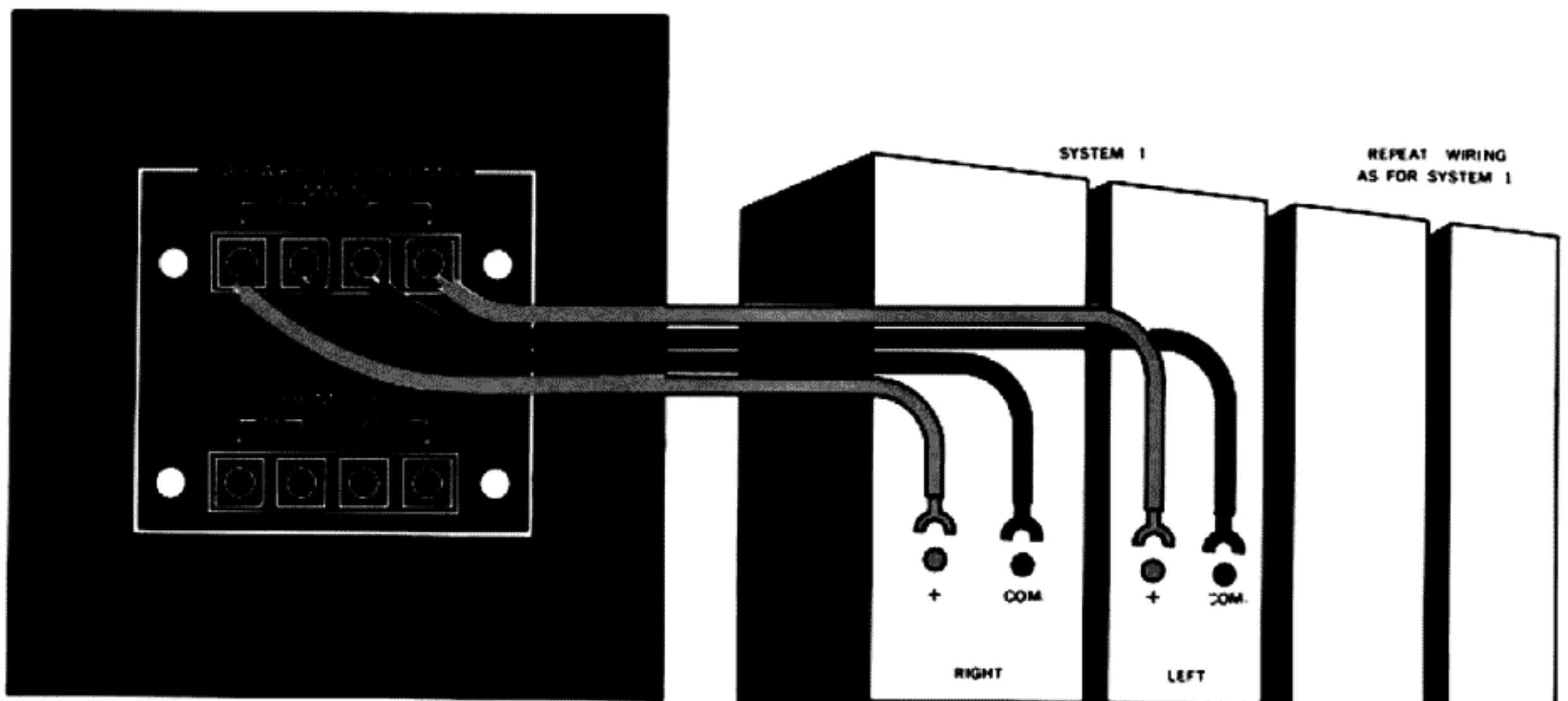
Figure 2. Loudspeaker System Connections
