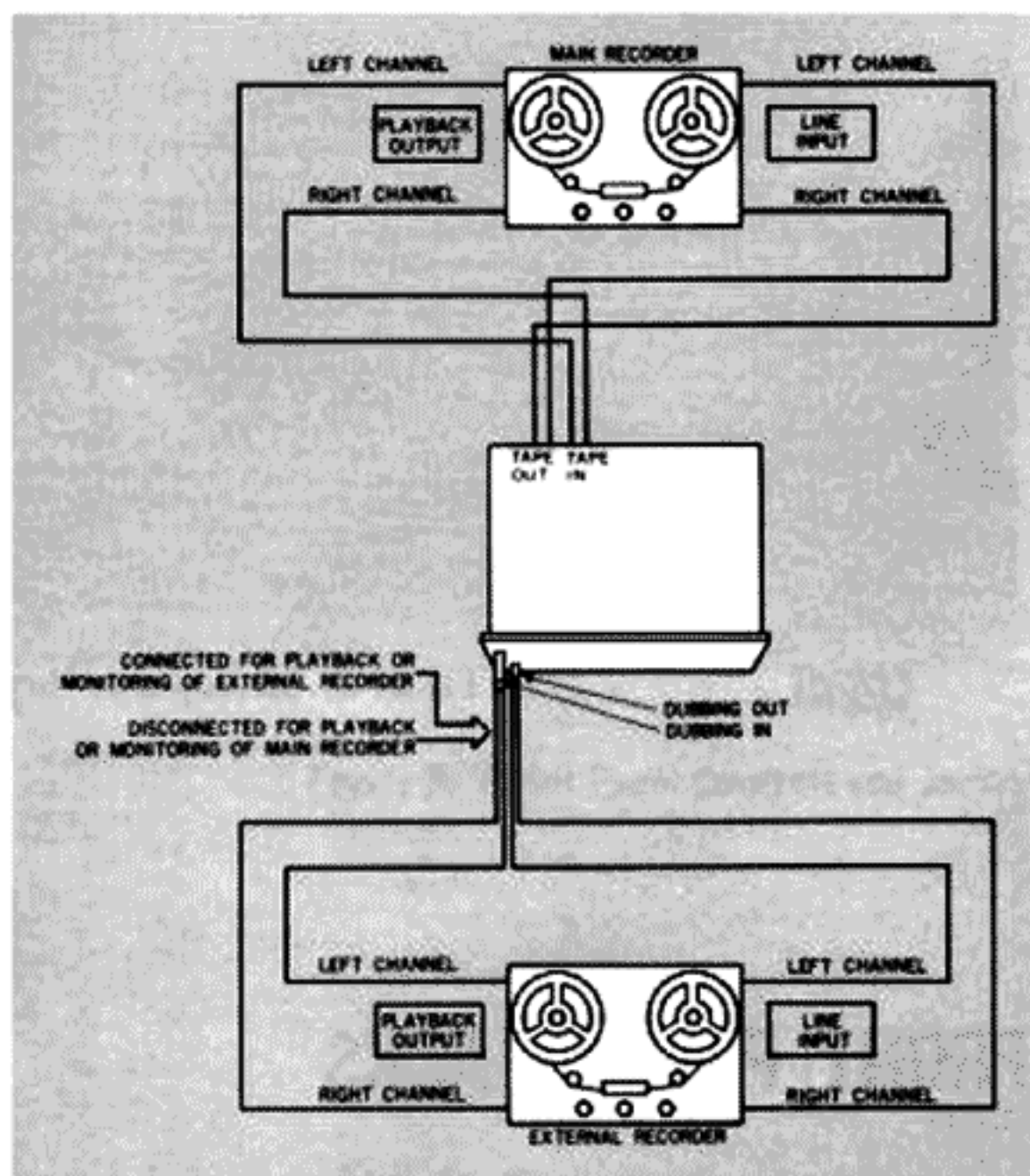
Figure 7. Arrangement of Two Tape Recorder
