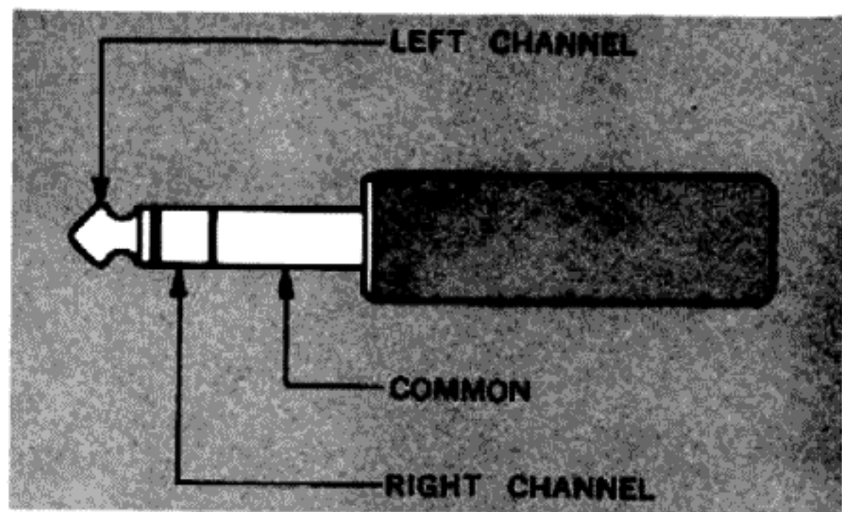
Figure 6. Stereophone Plug
